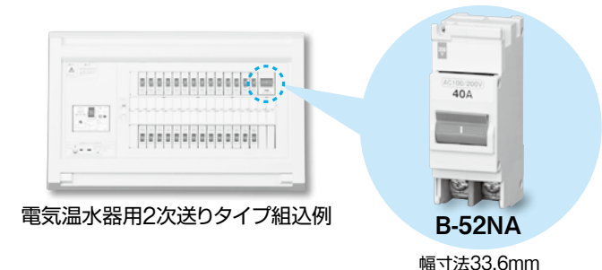
幅寸法33.6mm
