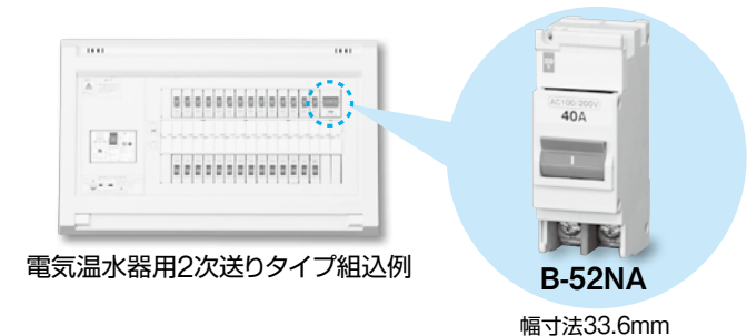
幅寸法33.6mm
