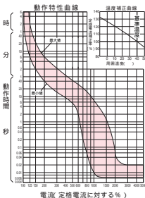
GB-72EC, GB-73EC
