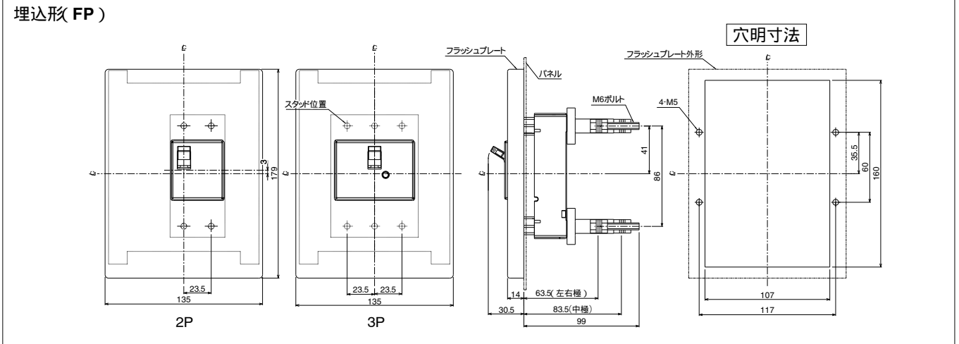
B-32EC(15, 20, 30A), B-33EC B-52EC(15, 20, 30A), B-53EC(15, 20, 30A)
