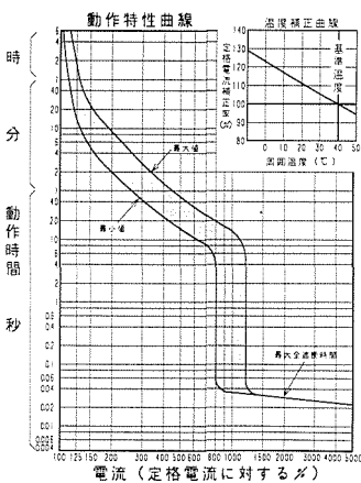
20 GB-403FA
