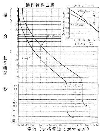
13 GB-403S, GBU-403-1S
