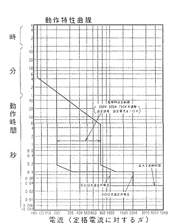
21 GB-603FA
