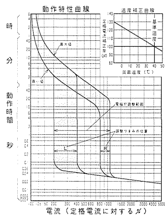
21 GB-603F
