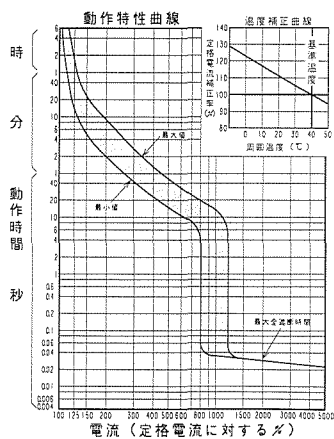
20 GB-403FA
