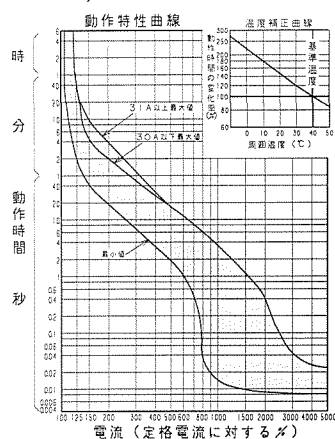
18 GB-63FK, GB-103FKA
