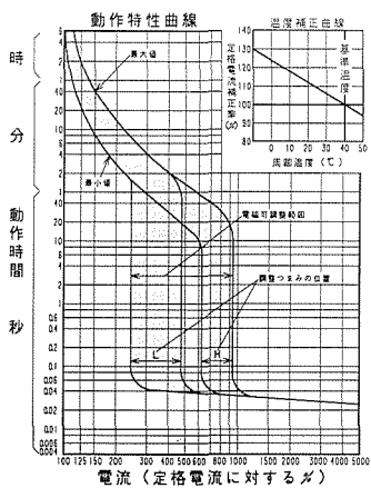
23 GB-1003F
